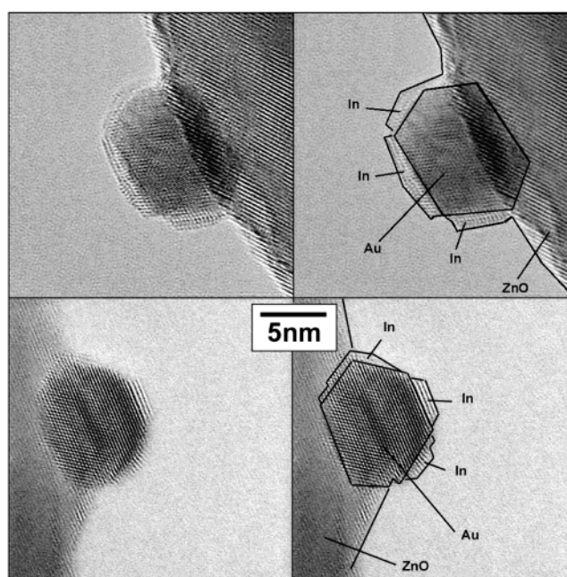
Figure 5. HRTEM images of Au–In/ZnO (left) plus same area with indicated structures (left).
